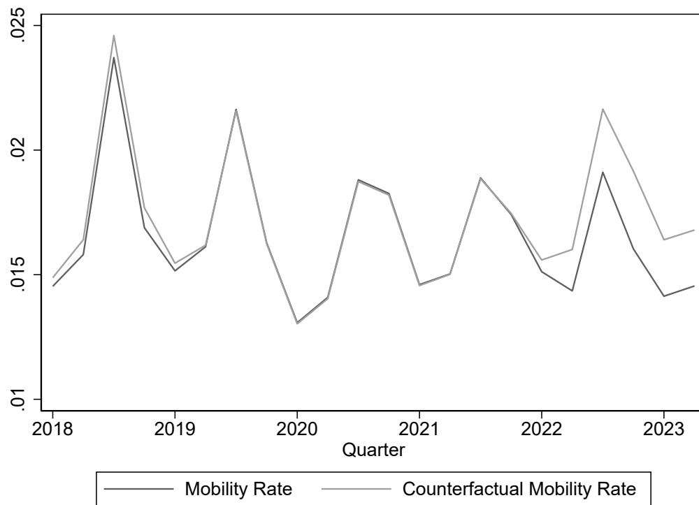
Figure B.1: Actual and Counterfactual Quarterly ZIP Code Moving Hazards
